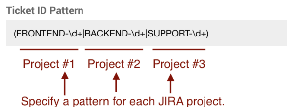
Fig. 5.37: Ticket ID specification that matches items from multiple JIRA projects.
