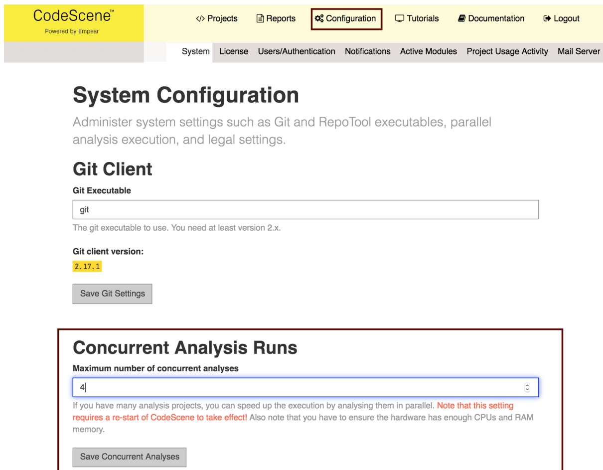
Fig. 5.40: Configure the maximum number of concurrent analyses.
