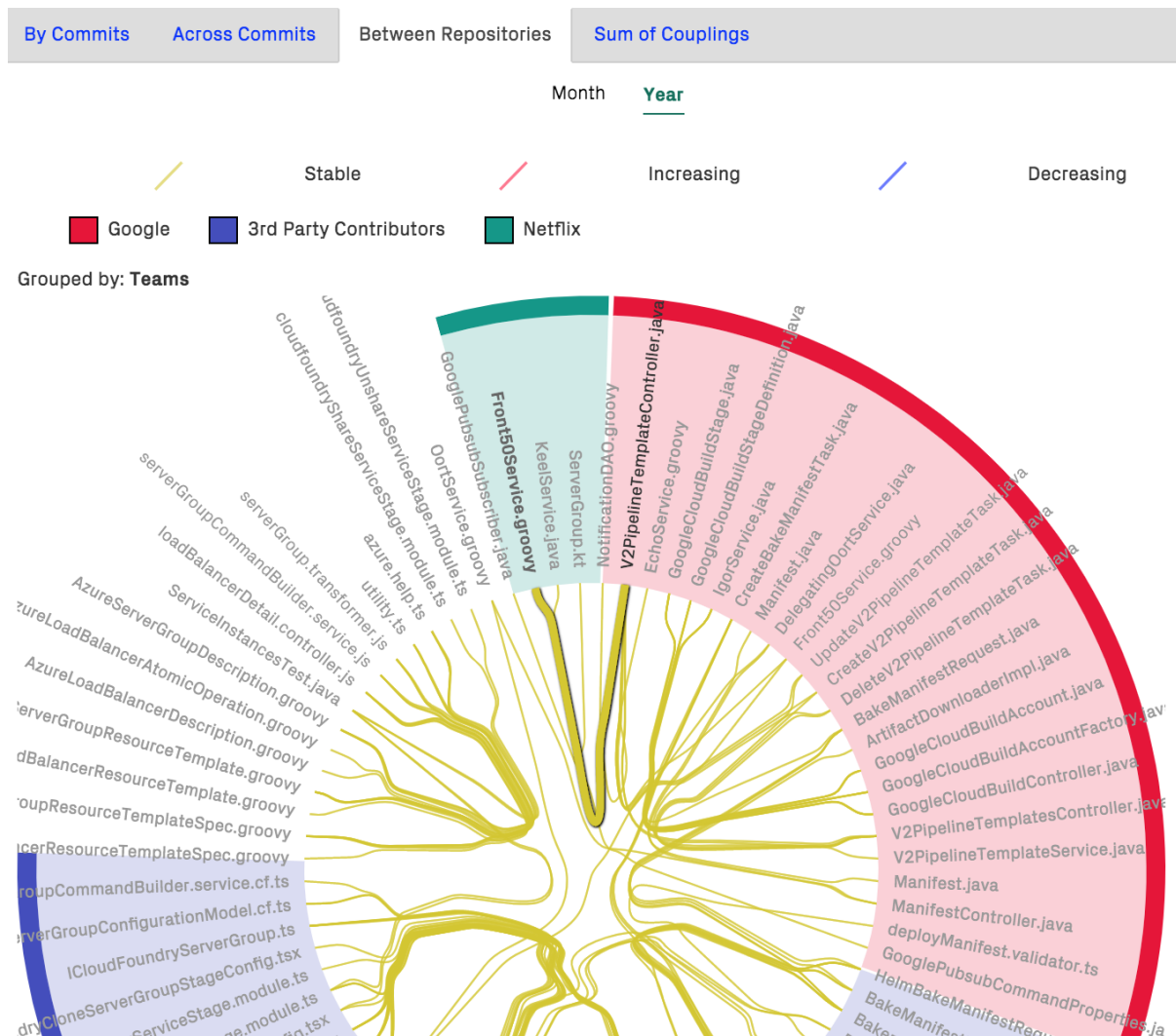
Fig. 4.38: Visualizing logical dependencies across team boundaries (example from Spinnaker).
