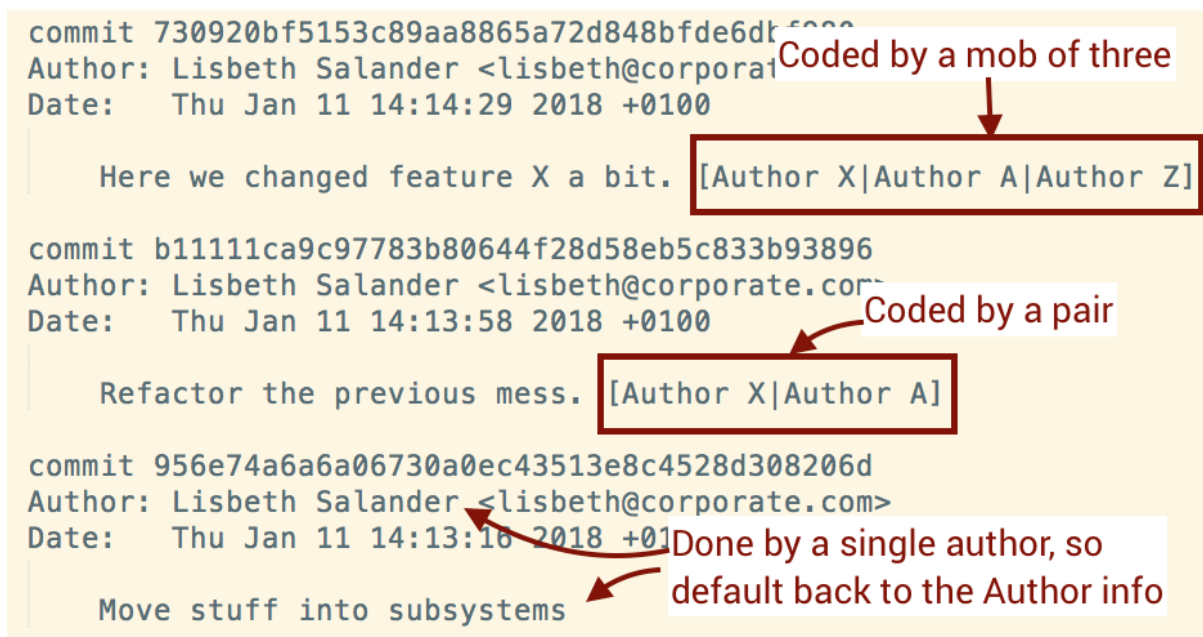
Fig. 5.29: Pair and mob programming annotations in the commit messages.
