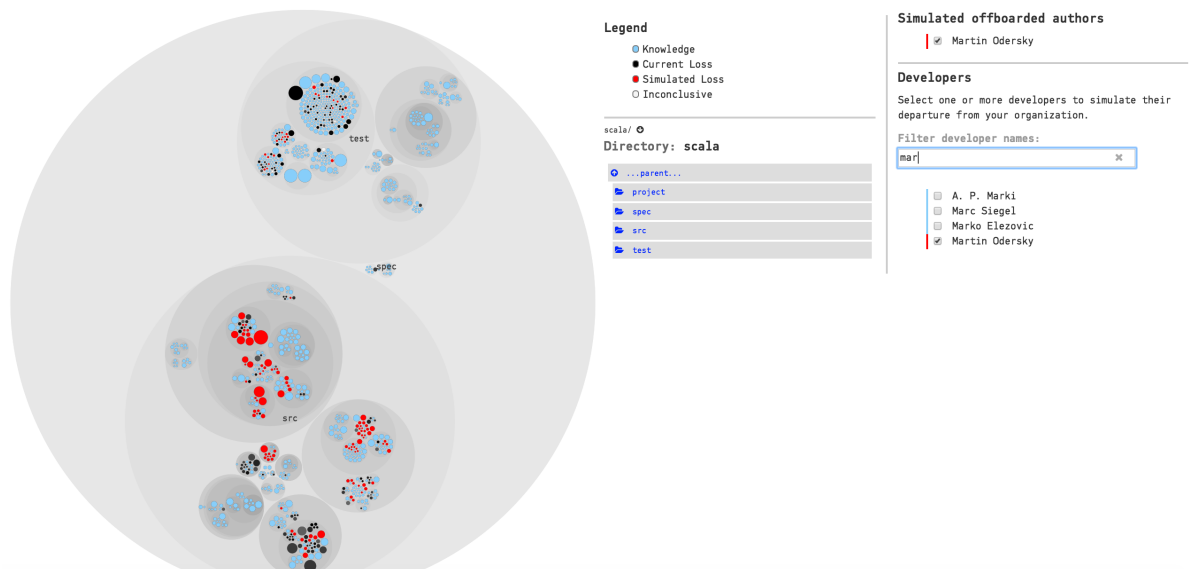
Fig. 4.138: Select one or more developers to simulate the off-boarding effect.
