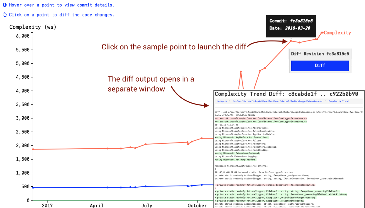
Fig. 4.44: Diff a complexity trend by clicking on a sample point.
