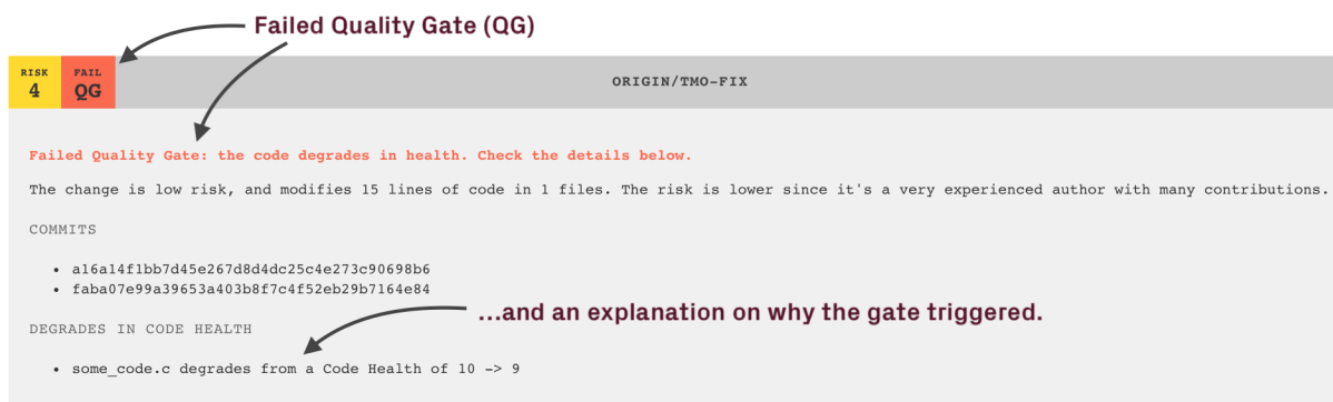
Fig. 4.121: A Delta Analysis detects degrading Code Health.
