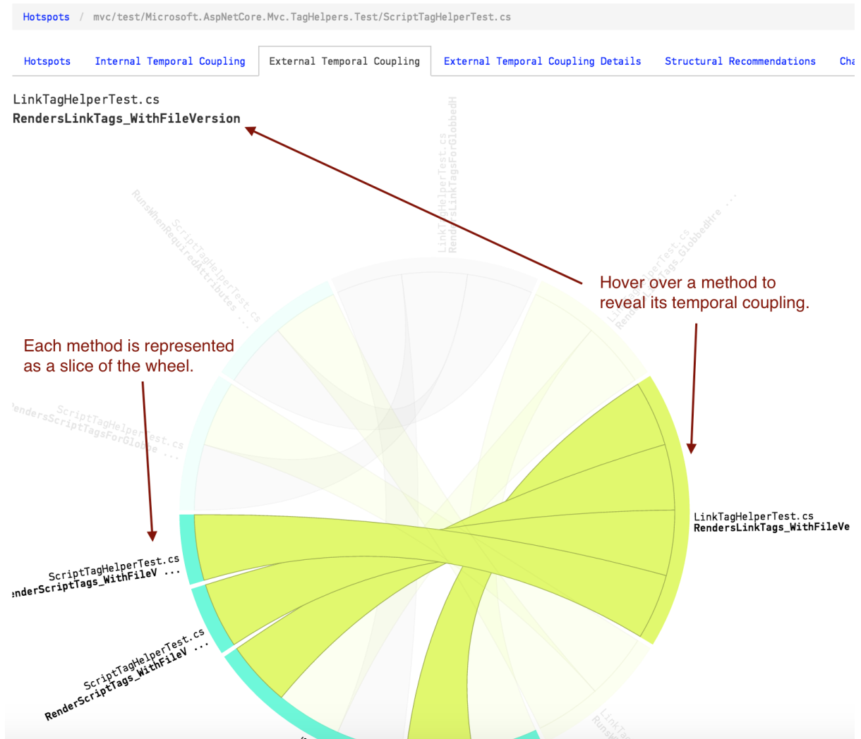
Fig. 4.52: The dependency wheel shows the temporal coupling between methods.
