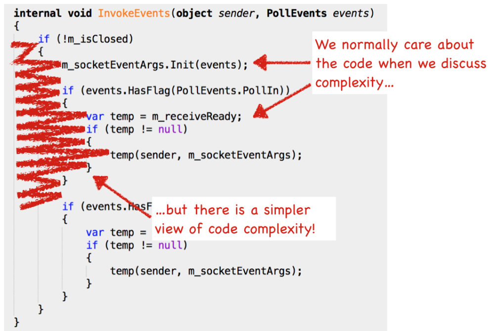
Fig. 4.46: Explaining whitespace complexity.
