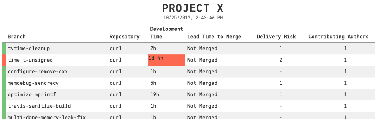
Fig. 1.14: Predict the delivery risk of each branch.
