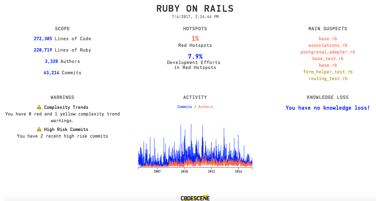
Fig. 1.12: The monitor dashboard gives you a high-level overview of your codebase.
