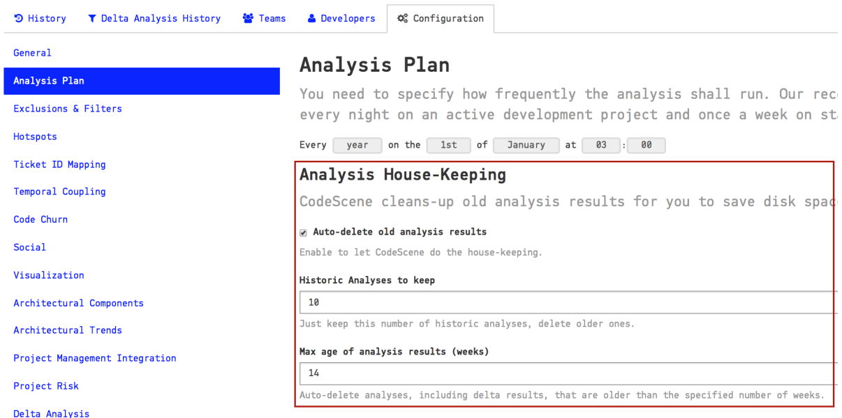
Fig. 5.5: Specify how much history you want to keep.
