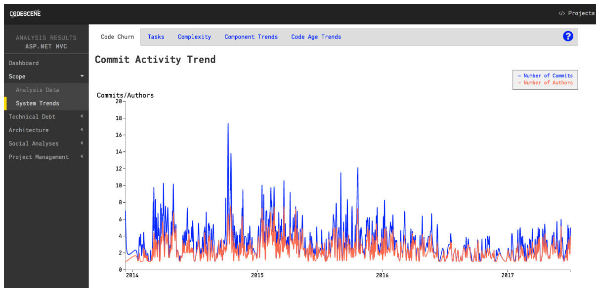
Fig. 4.58: The commit activity chart.
