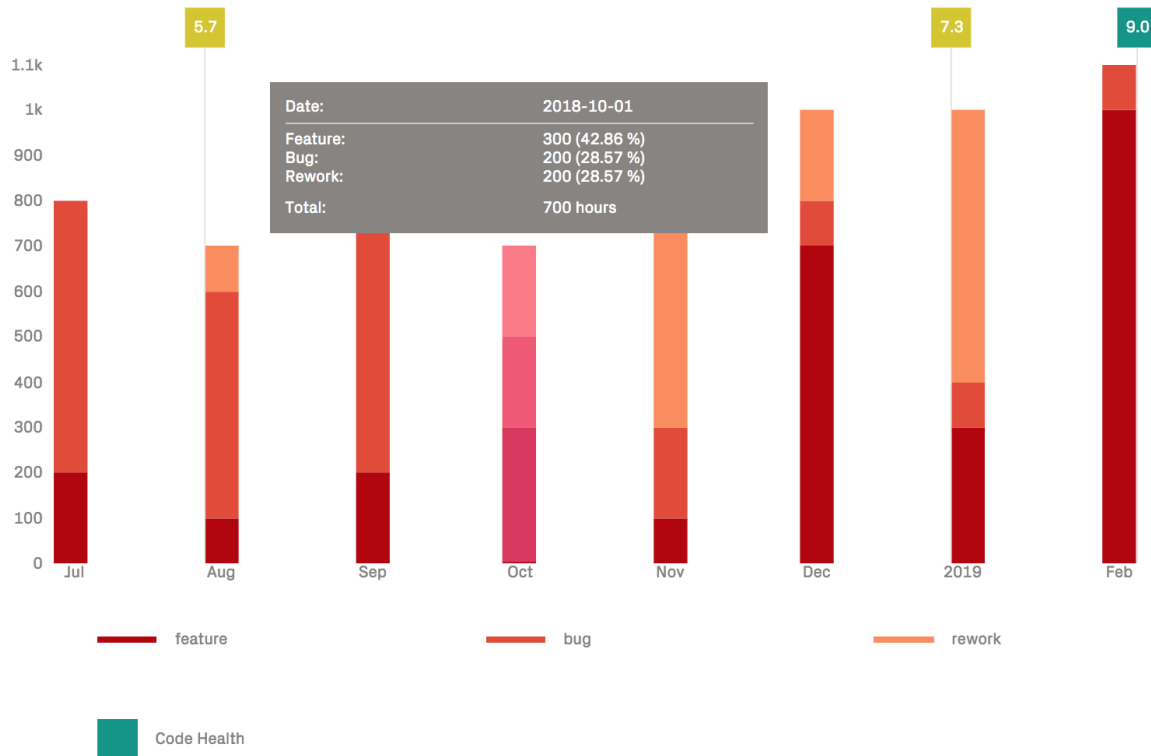
Fig. 3.2: CodeScene calculates cost trends on a file-, architecture-, and system-level.
