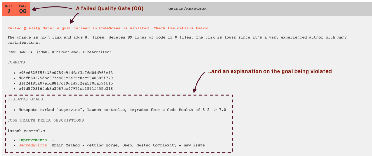
Fig. 2.7: Your goals are supervised in the CI/CD pipeline.
