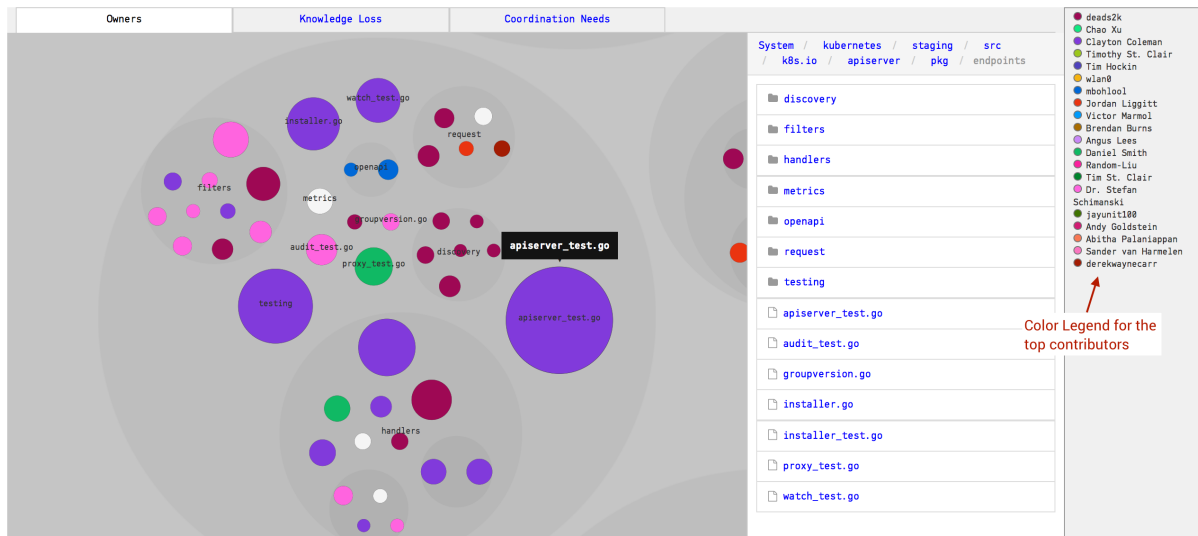
Fig. 4.95: An example of a knowledge map, click on a circle to get more information.
