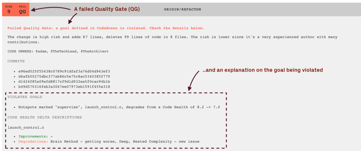
Fig. 4.120: A Delta Analysis gives you early warnings, actionable quality gates, and detects high risk changes (example from Jenkins).
