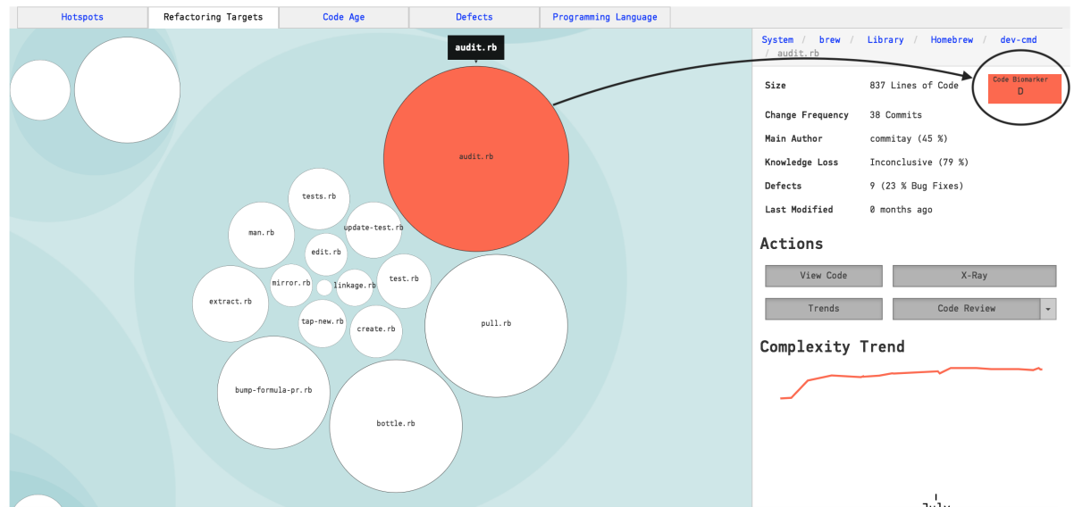
Fig. 4.8: CodeScene prioritizes the Hotspots in your code.
