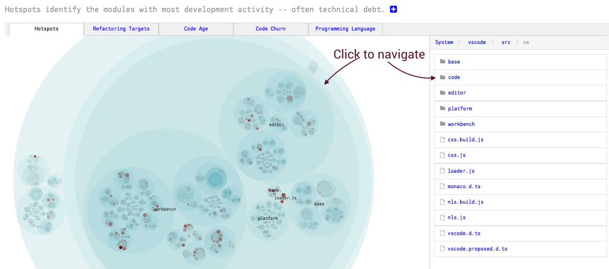
Fig. 4.6: Hotspots in the Visual Studio Code codebase.
