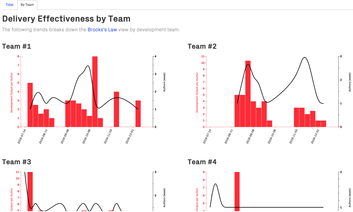
Fig. 4.90: Trends in development output for each team.
