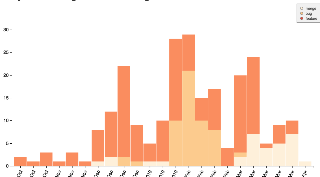
Fig. 4.108: Inspect all commits that mention a particular word or phrase.
