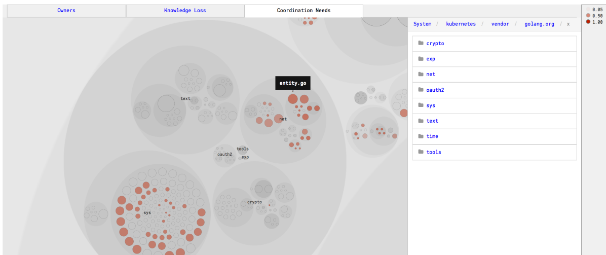
Fig. 4.98: The coordination needs between your development teams.
