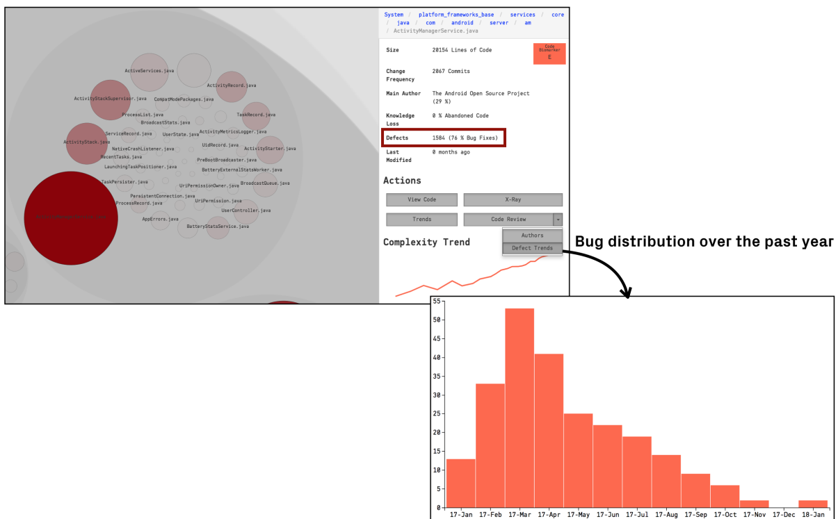
Fig. 4.13: The distribution of bug fixes over the past year.
