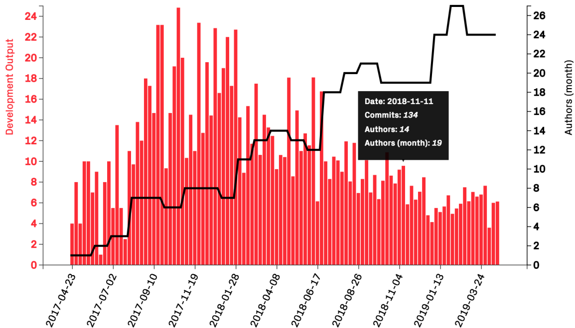
Fig. 4.89: Trends in development output with respect to the number of contributing authors.
