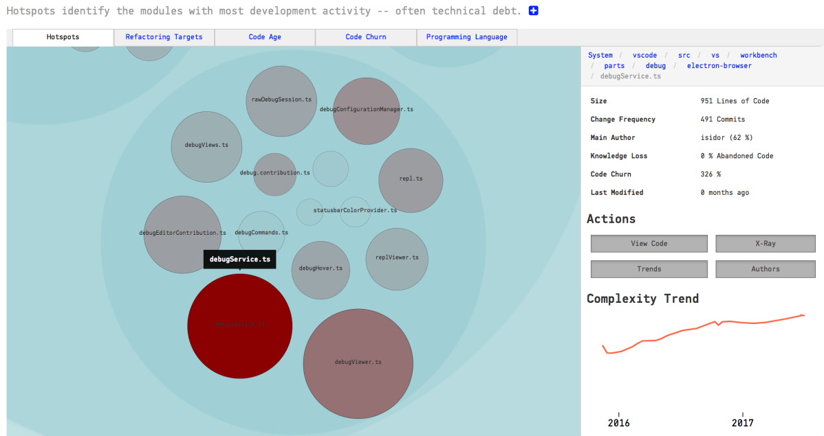
Fig. 4.16: Click on a Hotspot to access the context menu.
