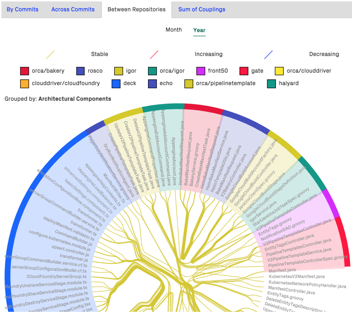
Fig. 4.84: Change coupling between files implemented in different programming languages and located in separate Git repositories.
