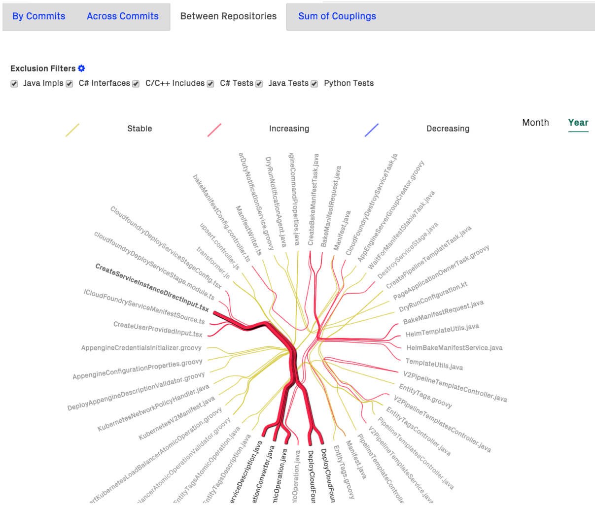
Fig. 4.36: Hover over a file in the change coupling graph to see its dependants.
