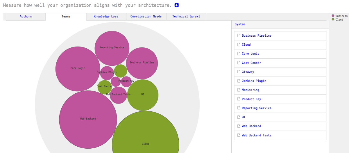
Fig. 4.67: High level architectural analyses on the technical and social aspects of code.
