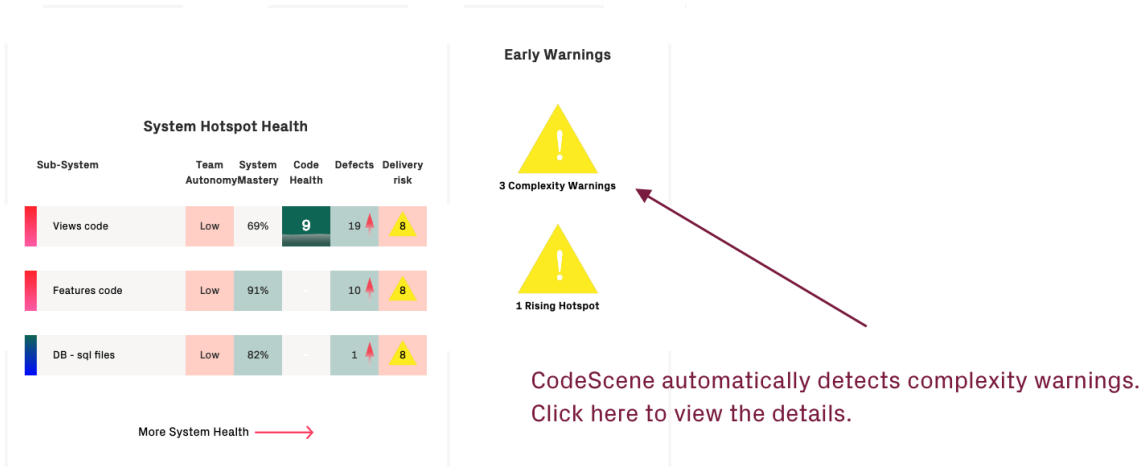
Fig. 4.43: CodeScene supervises your complexity trends.
