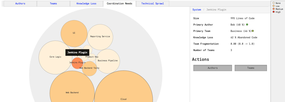
Fig. 4.86: Find team coordination bottlenecks.
