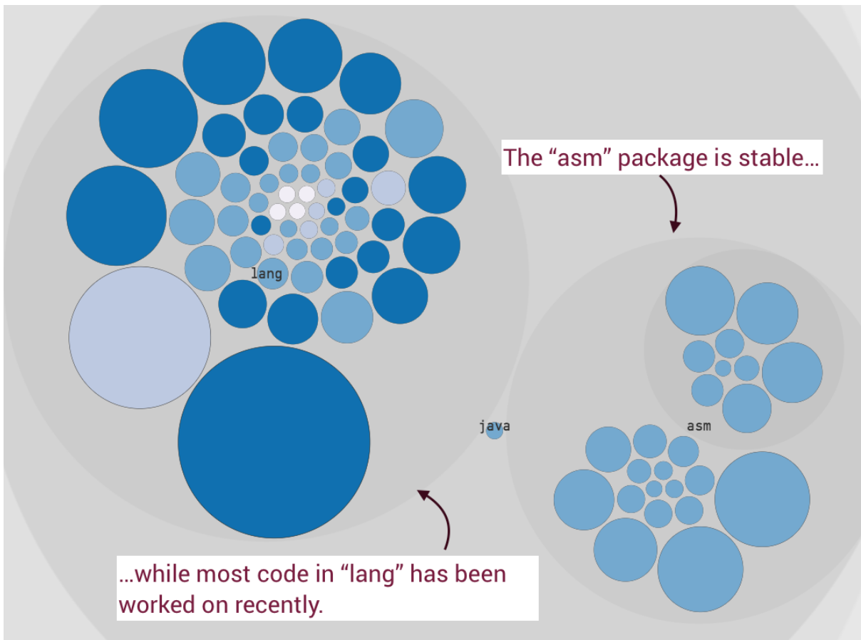
Fig. 4.65: Stable code in Clojure.
