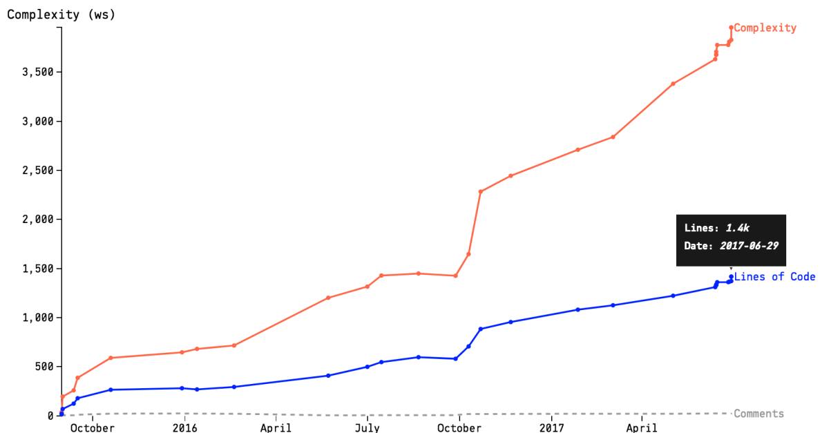
Fig. 4.39: A complexity trend sample.
