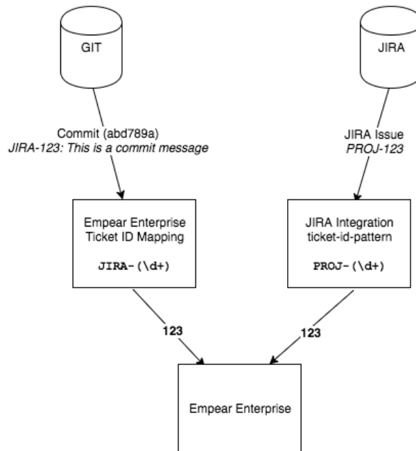
Fig. 5.36: Ticket IDs are extracted from the VCS logs using Ticket ID Mapping, and Project Management Item IDs are mapped from JIRA issue keys using a configured pattern in the JIRA integration service.
