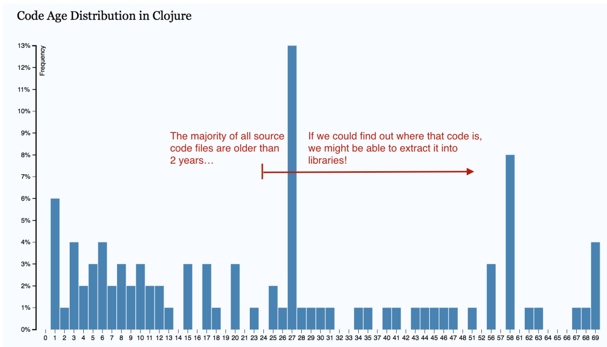
Fig. 4.63: Code age distribution in Clojure.
