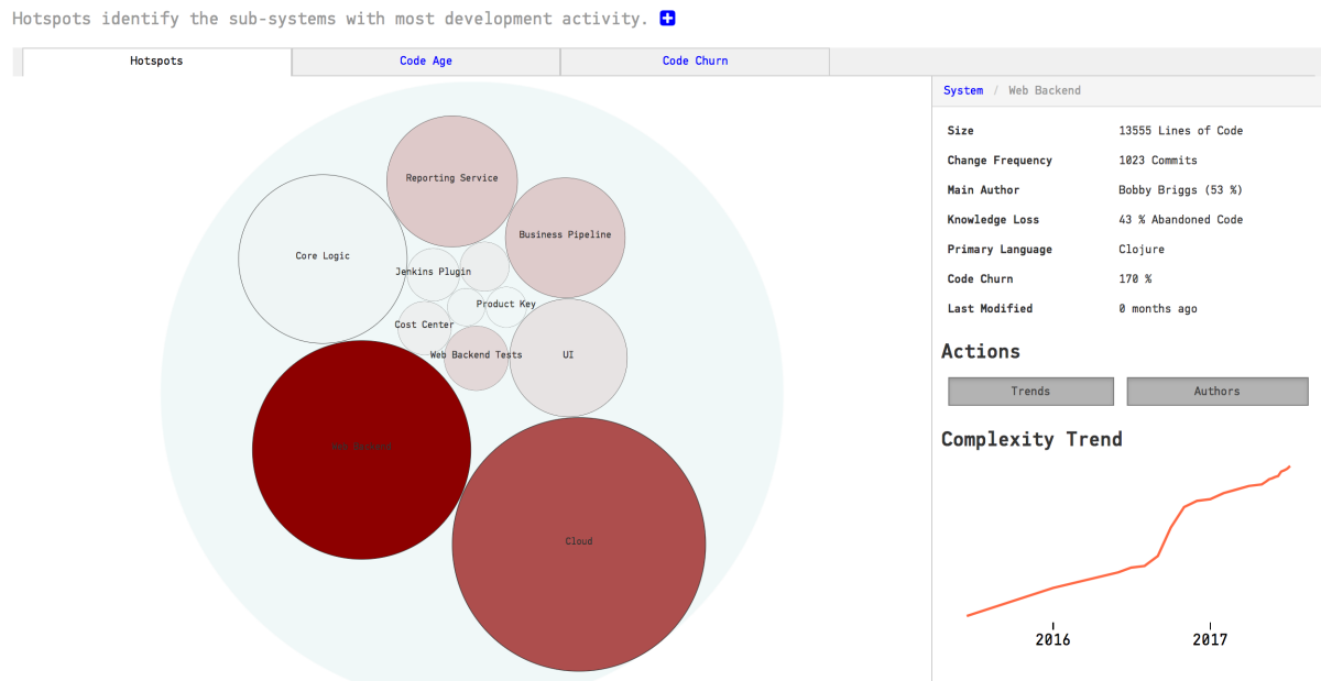
Fig. 4.70: High level architectural hotspots analysis.
