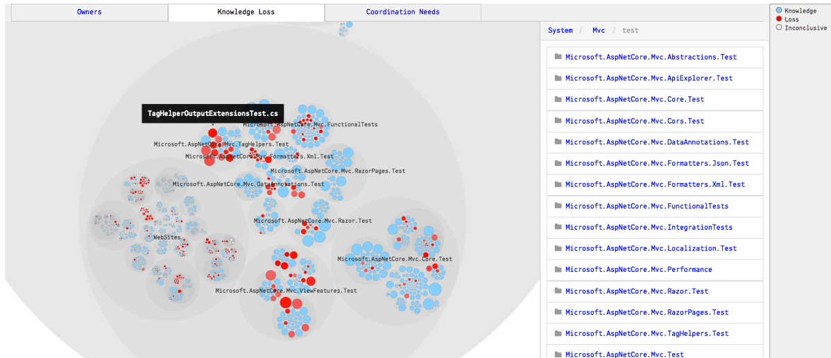
Fig. 4.103: An example on a knowledge loss analysis.
