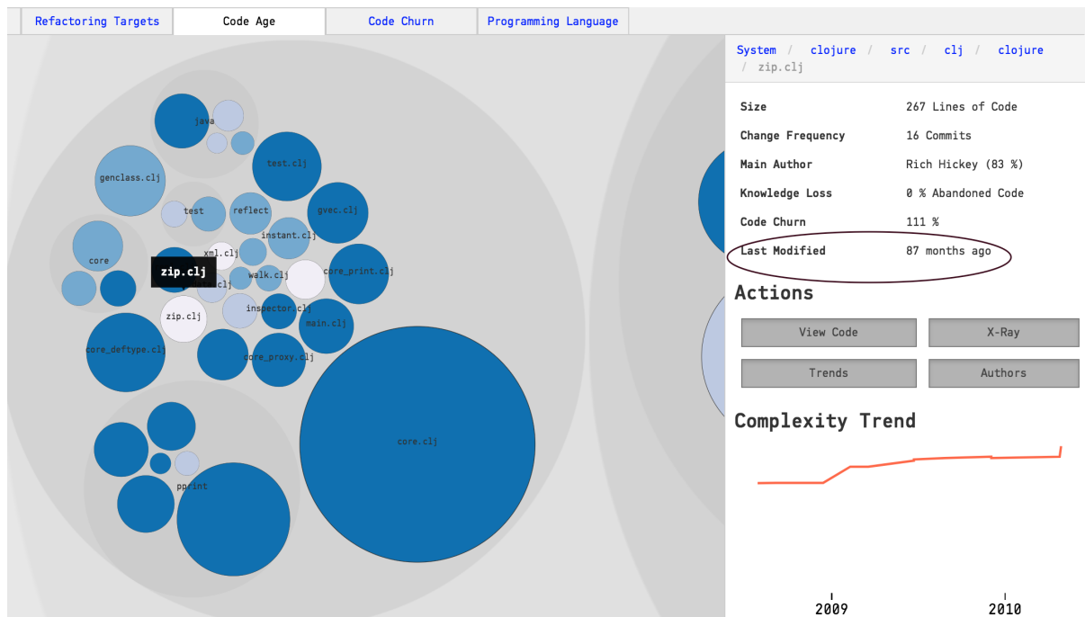
Fig. 4.66: Code that stabilizes at different rates.
