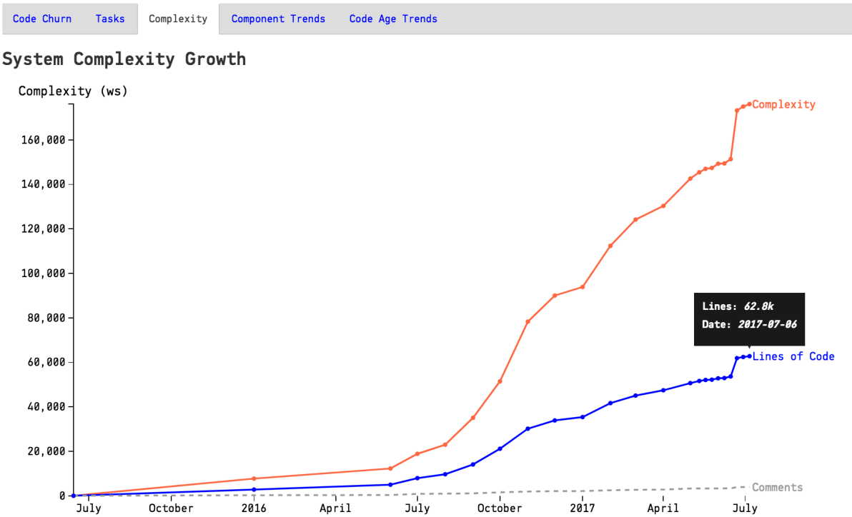
Fig. 4.80: The evolution of the complete codebase.
