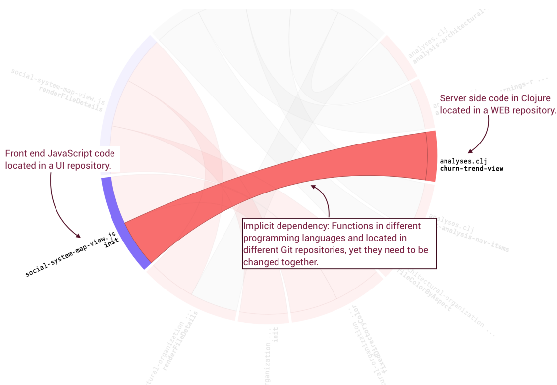
Fig. 4.53: X-Ray works across multiple repositories.
