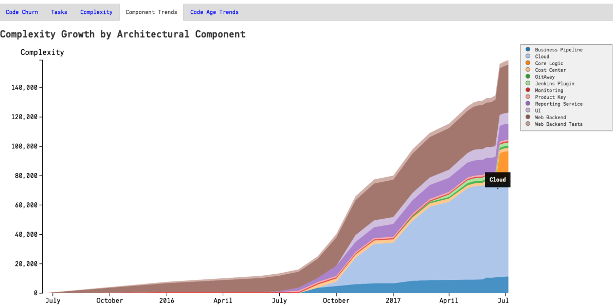
Fig. 4.81: The architectural trends let you view how the development effort has shifted over the years.
