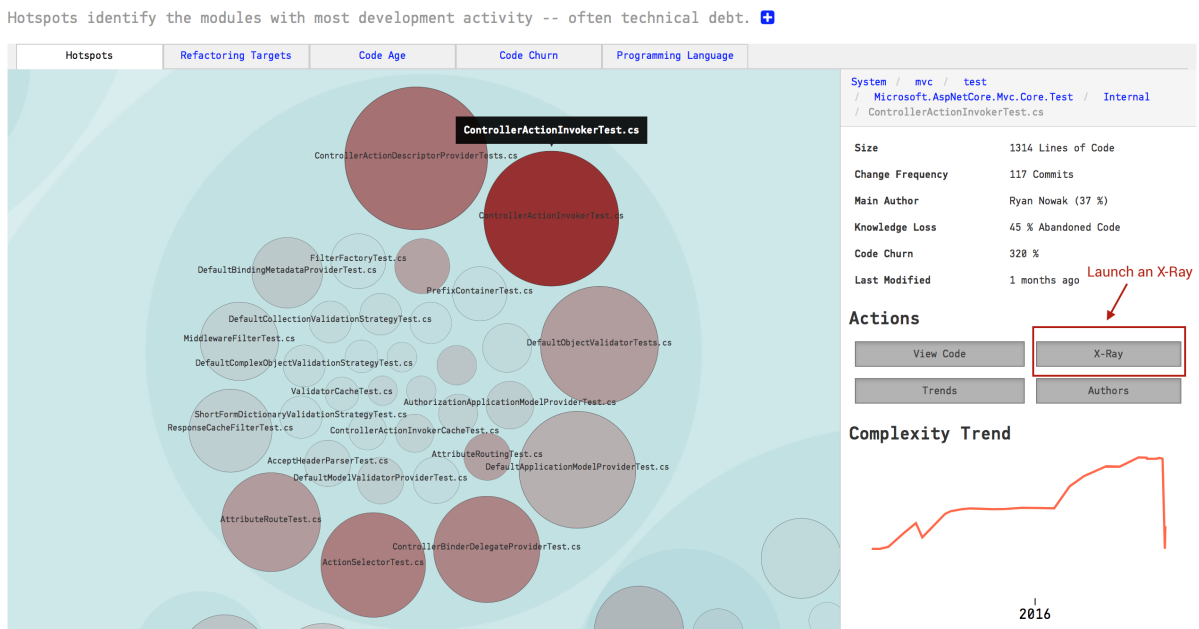
Fig. 4.47: Run X-Ray from the context menu.
