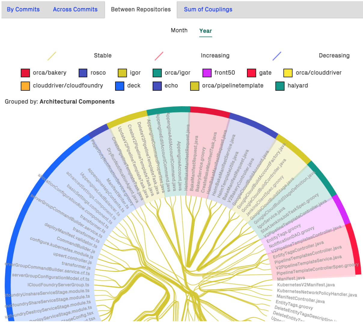
Fig. 4.37: Visualizing change coupling across microservices (example from Spinnaker).
