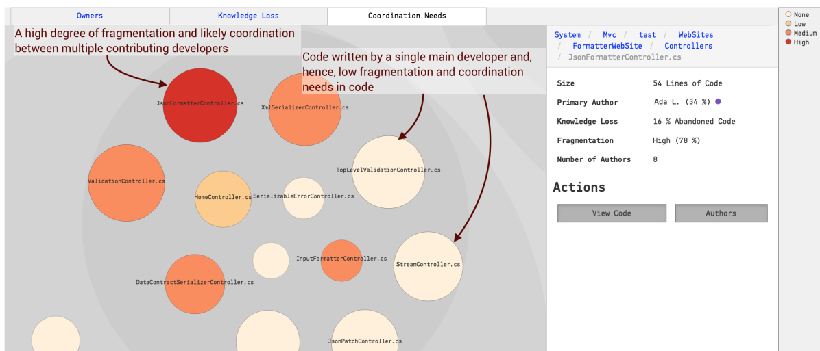
Fig. 4.105: The fragmentation map shows files with excess parallel development.
