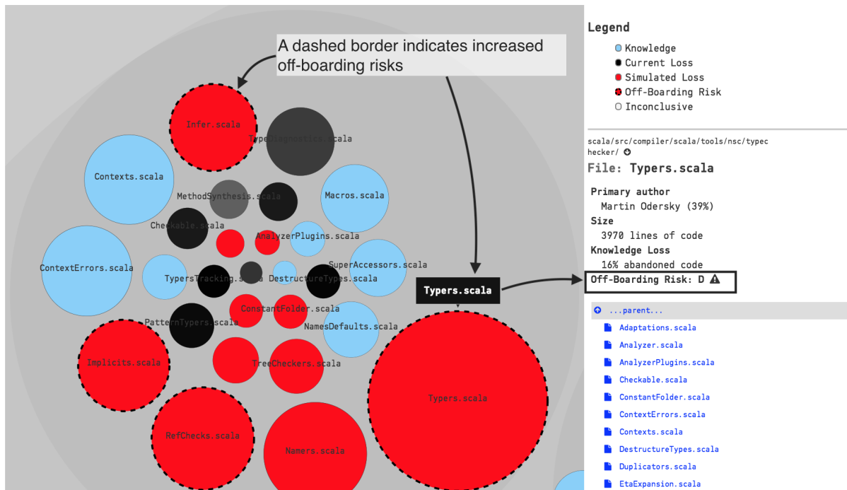
Fig. 4.139: CodeScene auto-detects off-boarding risks.
