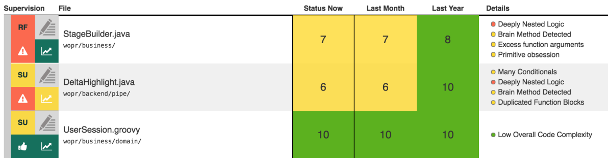
Fig. 4.22: Code Health Trends and Biomarkers for a specific project.
