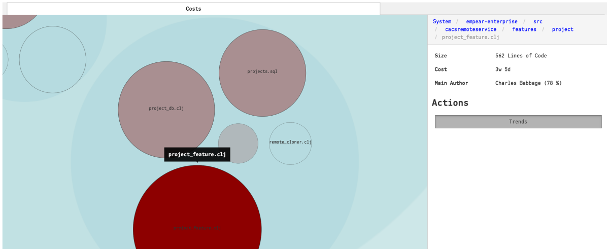
Fig. 4.112: A Hotspot analysis by cost lets you see where you spend most time.
