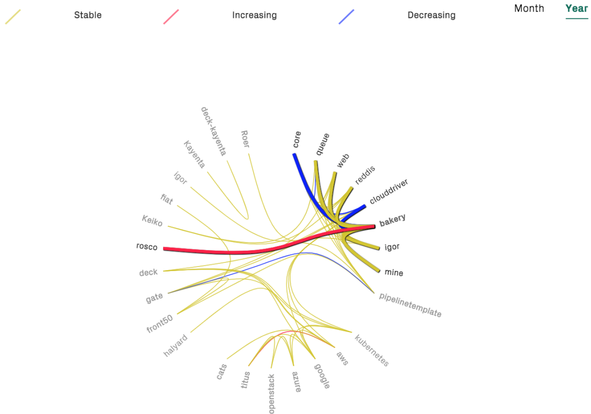
Fig. 4.83: Change coupling between different microservices.
