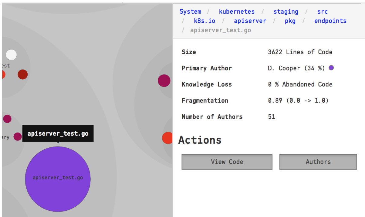
Fig. 4.96: Inspect the details of each file in the knowledge map.
