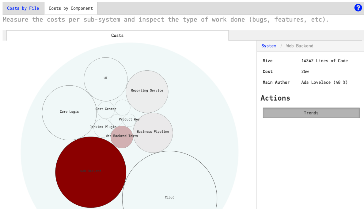
Fig. 4.115: Calculate hotspots by costs on architectural level
