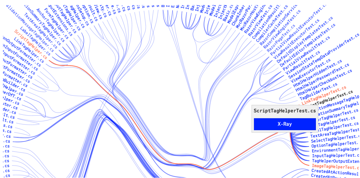
Fig. 4.51: X-Ray lets you investigate temporal coupling clusters in detail.
