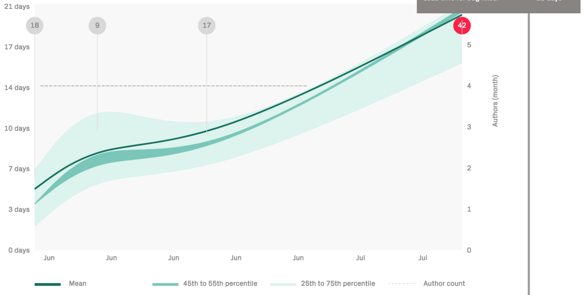
Fig. 4.132: Increasing lead times might indicate either organizational issues, planning problems, or growing technical debt.
