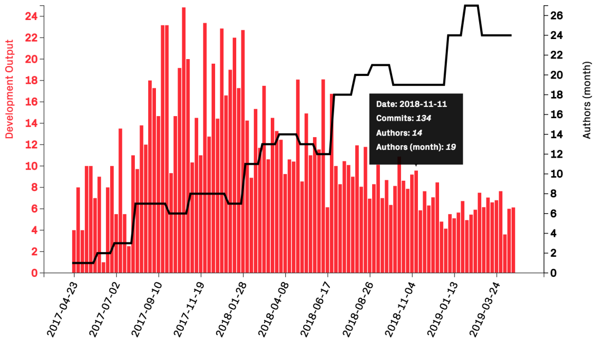
Fig. 3.92: Trends in development output with respect to the number of contributing authors.
