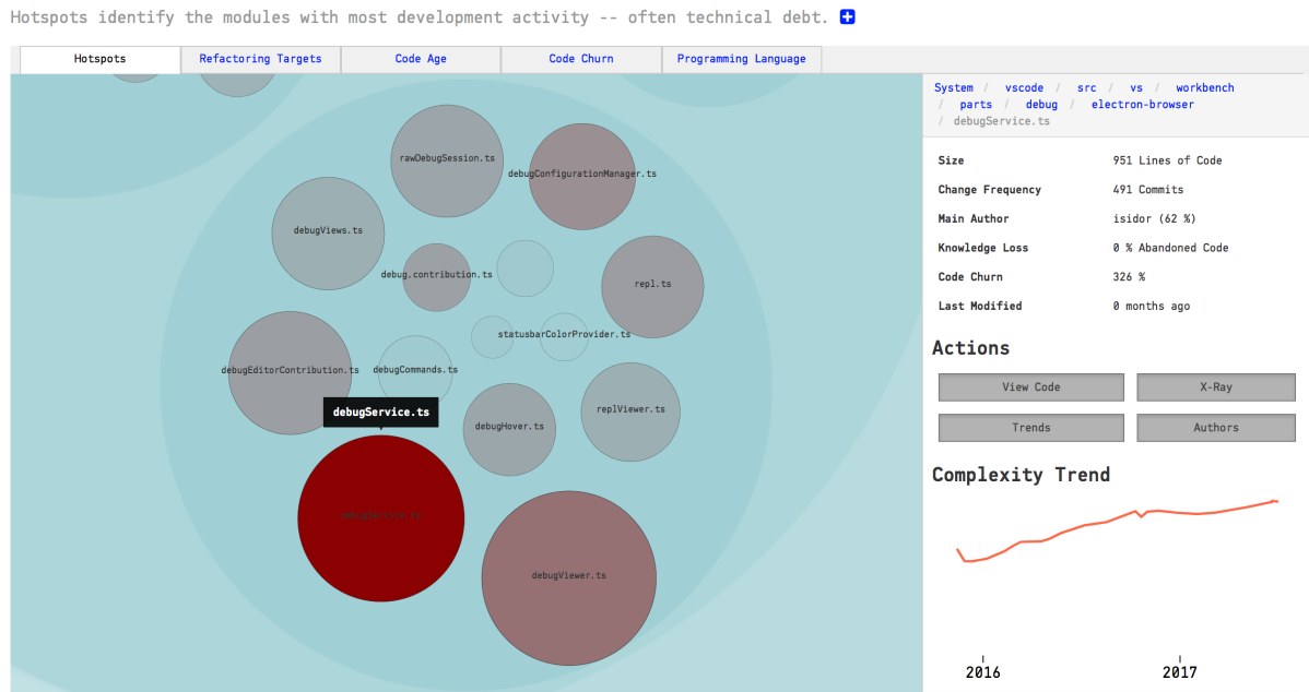
Fig. 3.16: Click on a Hotspot to access the context menu.
