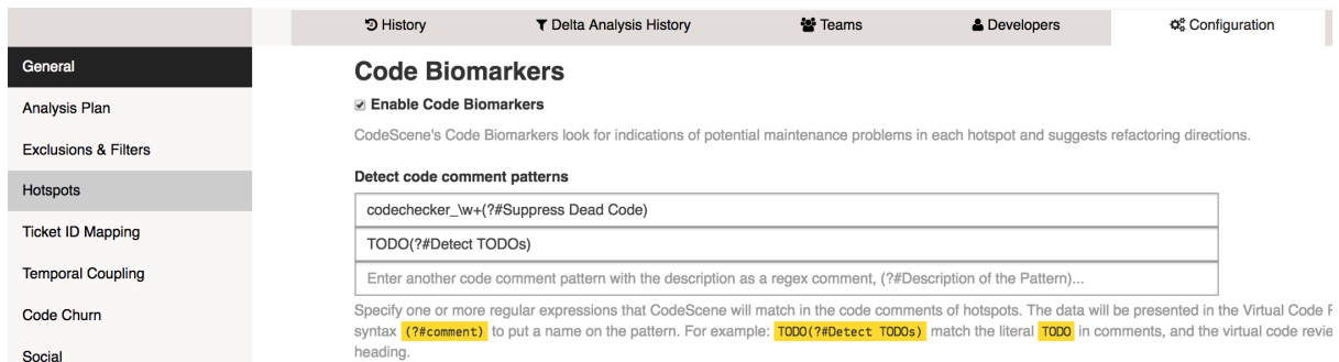
Fig. 4.10: Configure regular expressions to detect code comments.
