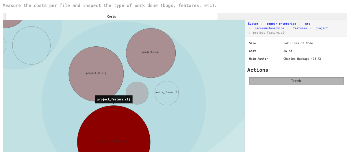
Fig. 3.109: A Hotspot analysis by cost lets you see where you spend most time.
