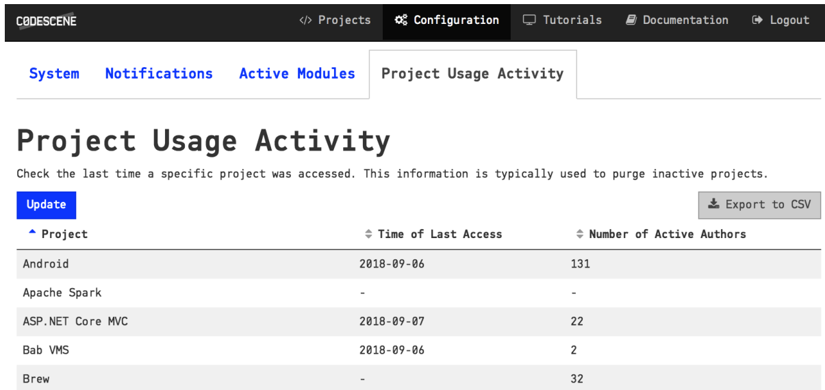
Fig. 4.38: A summary of the project usage activity in CodeScene.
