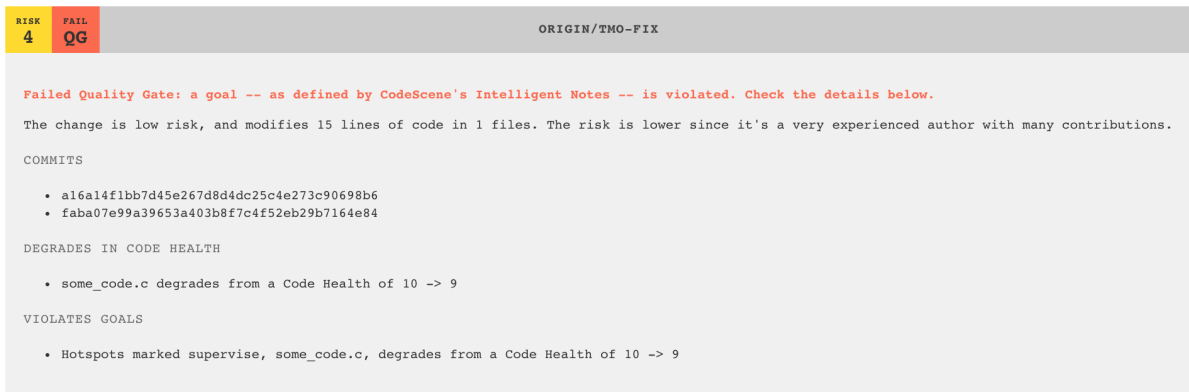
Fig. 3.116: A Delta Analysis gives you early warnings and detects high risk changes (example from Jenkins).
