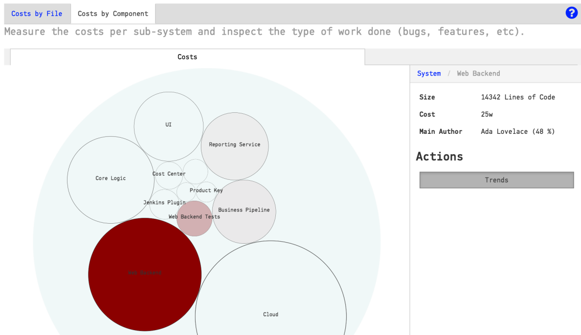
Fig. 3.112: Calculate hotspots by costs on architectural level
