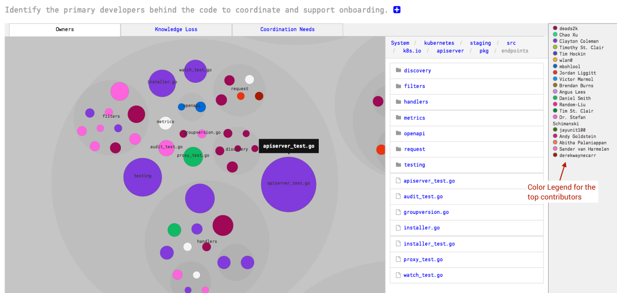
Fig. 3.95: An example of a knowledge map, click on a circle to get more information.
