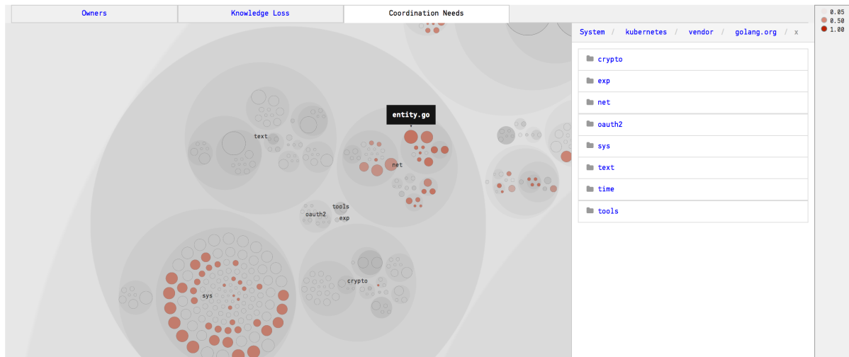
Fig. 3.98: The coordination needs between your development teams.
