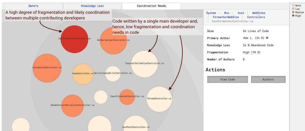
Fig. 3.102: The fragmentation map shows files with excess parallel development.
