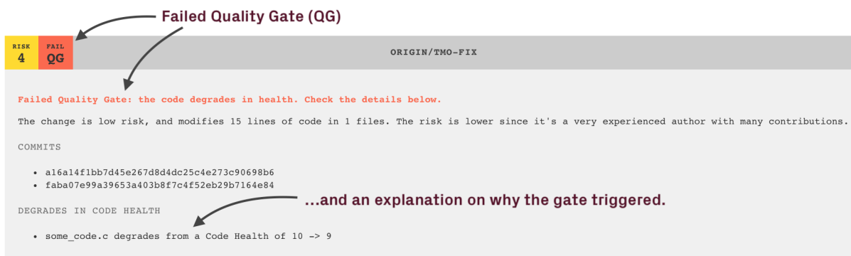
Fig. 3.117: A Delta Analysis detects degrading Code Health.
