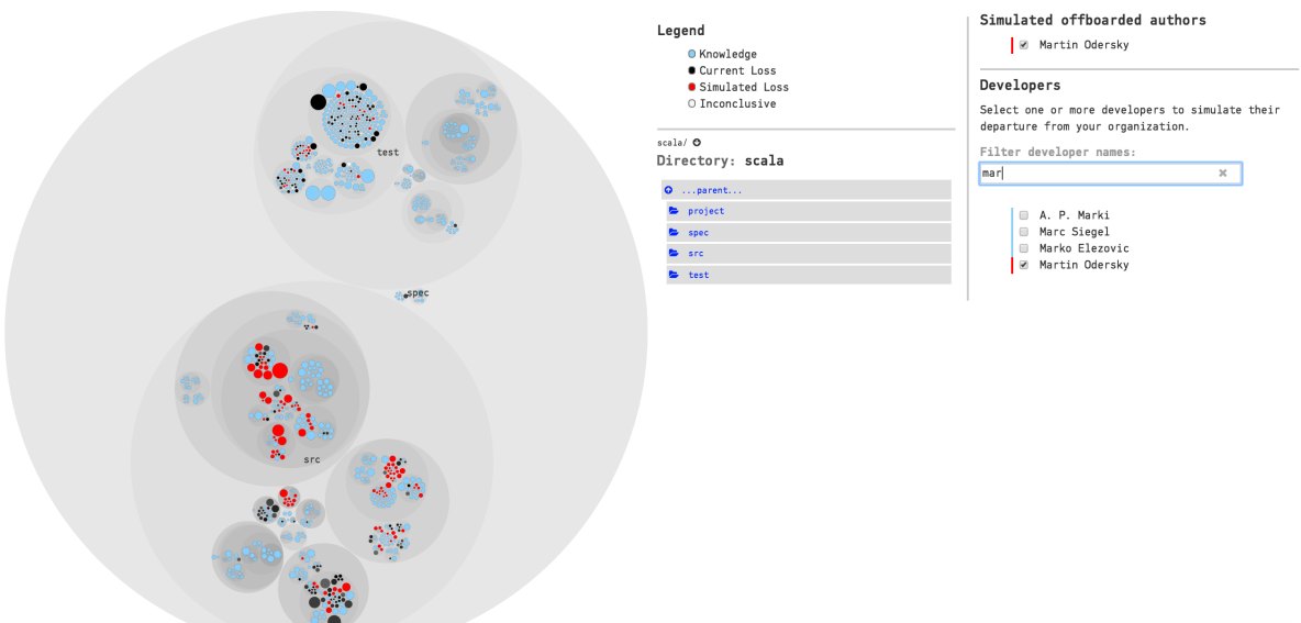
Fig. 3.125: Select one or more developers to simulate the off-boarding effect.
