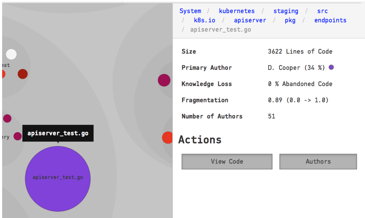
Fig. 3.96: Inspect the details of each file in the knowledge map.
