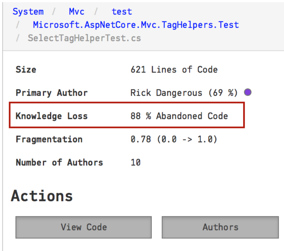
Fig. 3.101: Inspect the detailed knowledge loss of a file.
