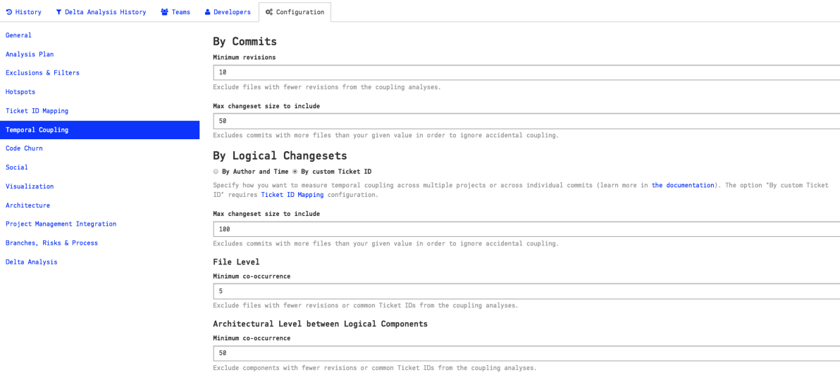
Fig. 3.42: Temporal coupling configuration.
