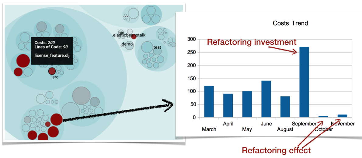
Fig. 3.111: Use the Cost Trends to measure the effect of improvements.
