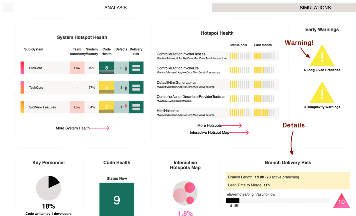
Fig. 3.121: An overview of the branch measures.
