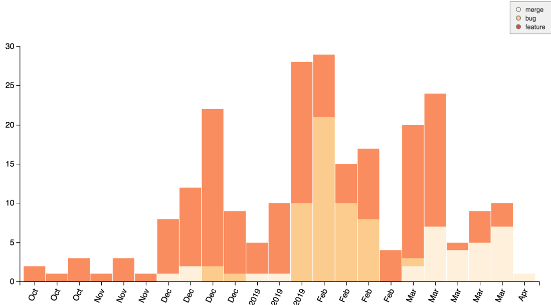
Fig. 3.105: Inspect all commits that mention a particular word or phrase.
