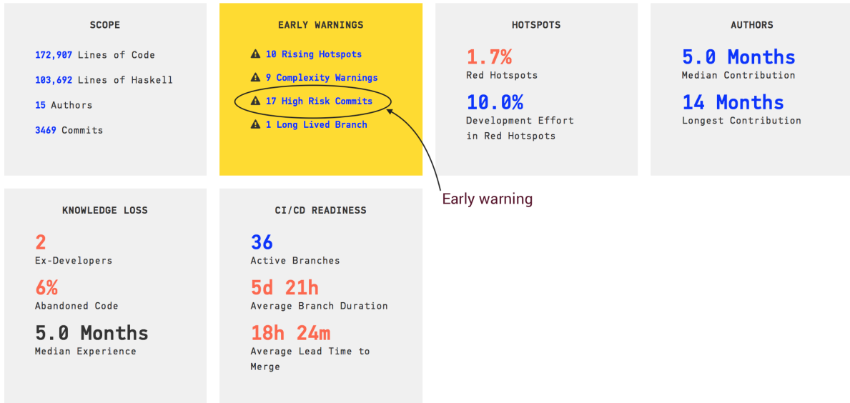
Fig. 3.113: An Early Warning for recent high risk commits.
